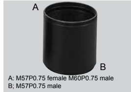
A: M57P0.75 female B: M57P0.75 male
