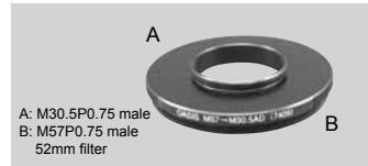
■ M57 to M30.5 AD [7409] Adapter for 30.5mm diameter threaded camera.
