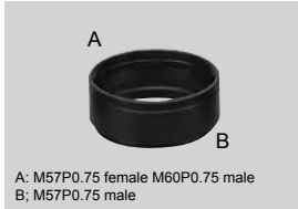
A: M57P0.75 female M60P0.75 male B: M57P0.75 male
