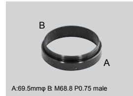
A: 69.5mmφ B: M68.8 P0.75 male
